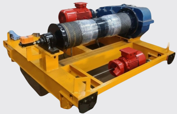
Crab Assembly
